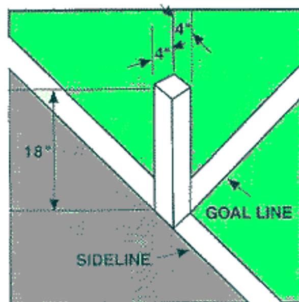
PYLON DETAIL
