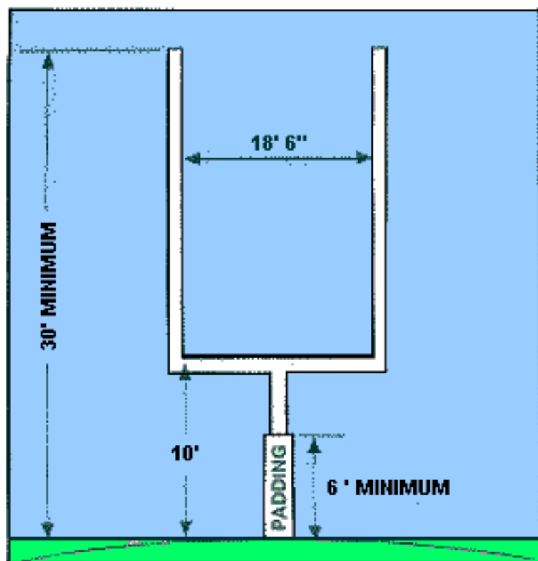
GOAL POST DETAIL
